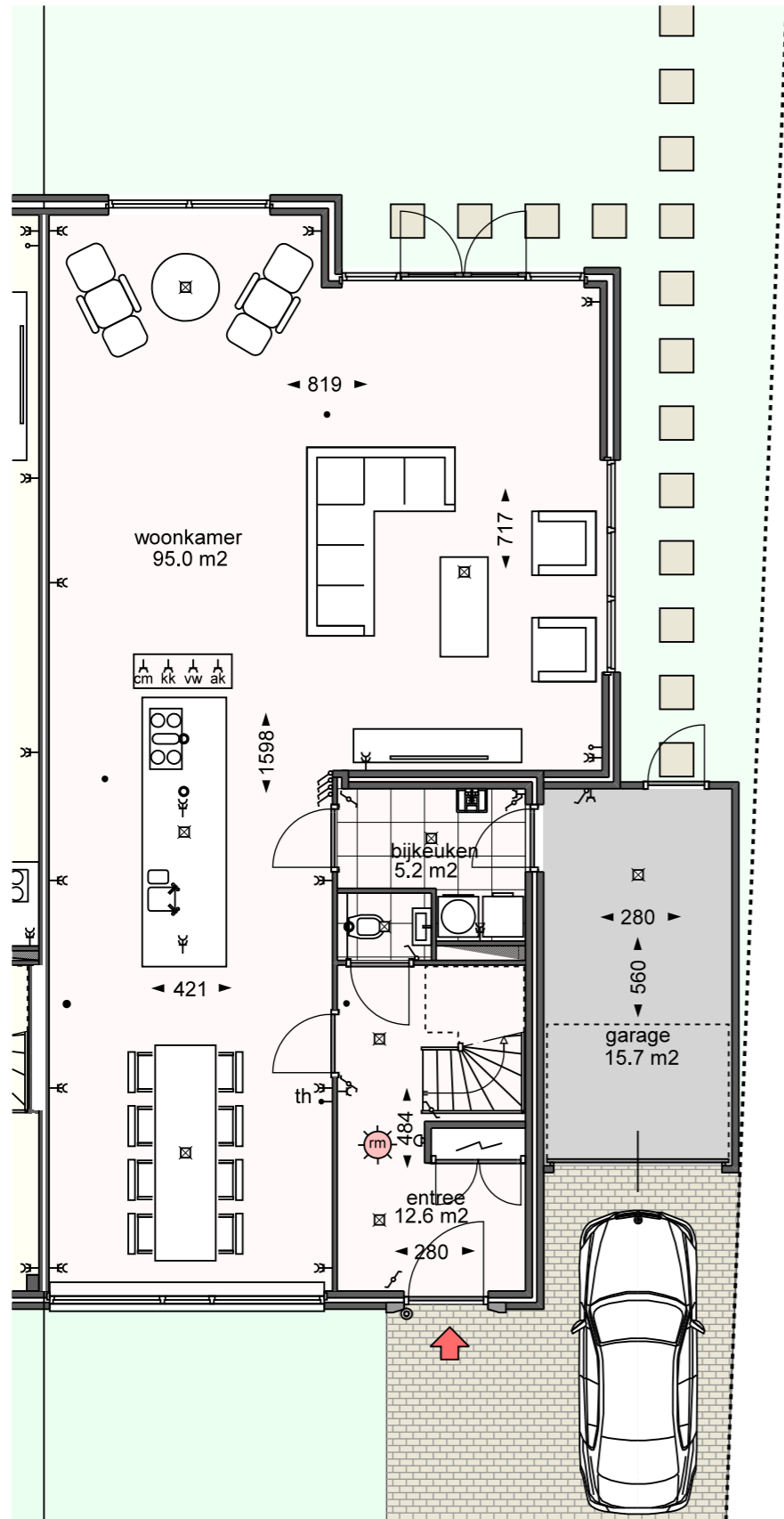
BEGANE GROND - 117 m 2 G.O. TYPE B
